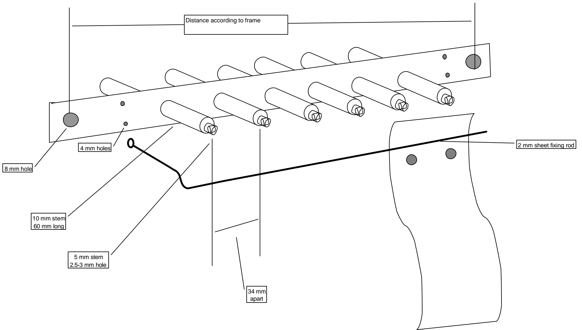
Sampler that can hold 6 sheets of each 100\text{cm}^2 . About 3 can be mounted in the sampler frame
